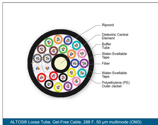
ALTOS® Loose Tube, Gel-Free Cable, 288 F, 50 µm multimode (OM3)
